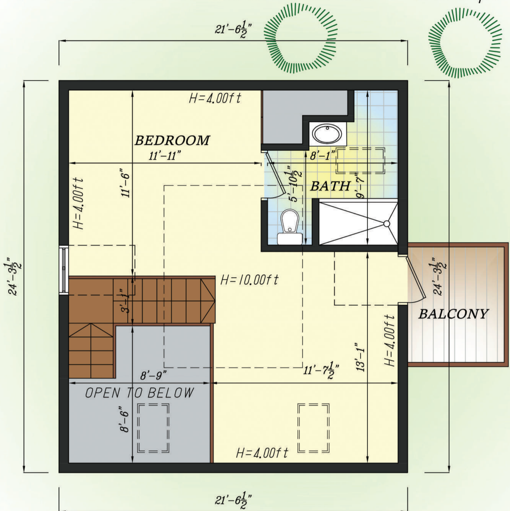
Upper Level Floor Plan Alicion - Carriage House 66 McDonald Street Lunenburg, NS
