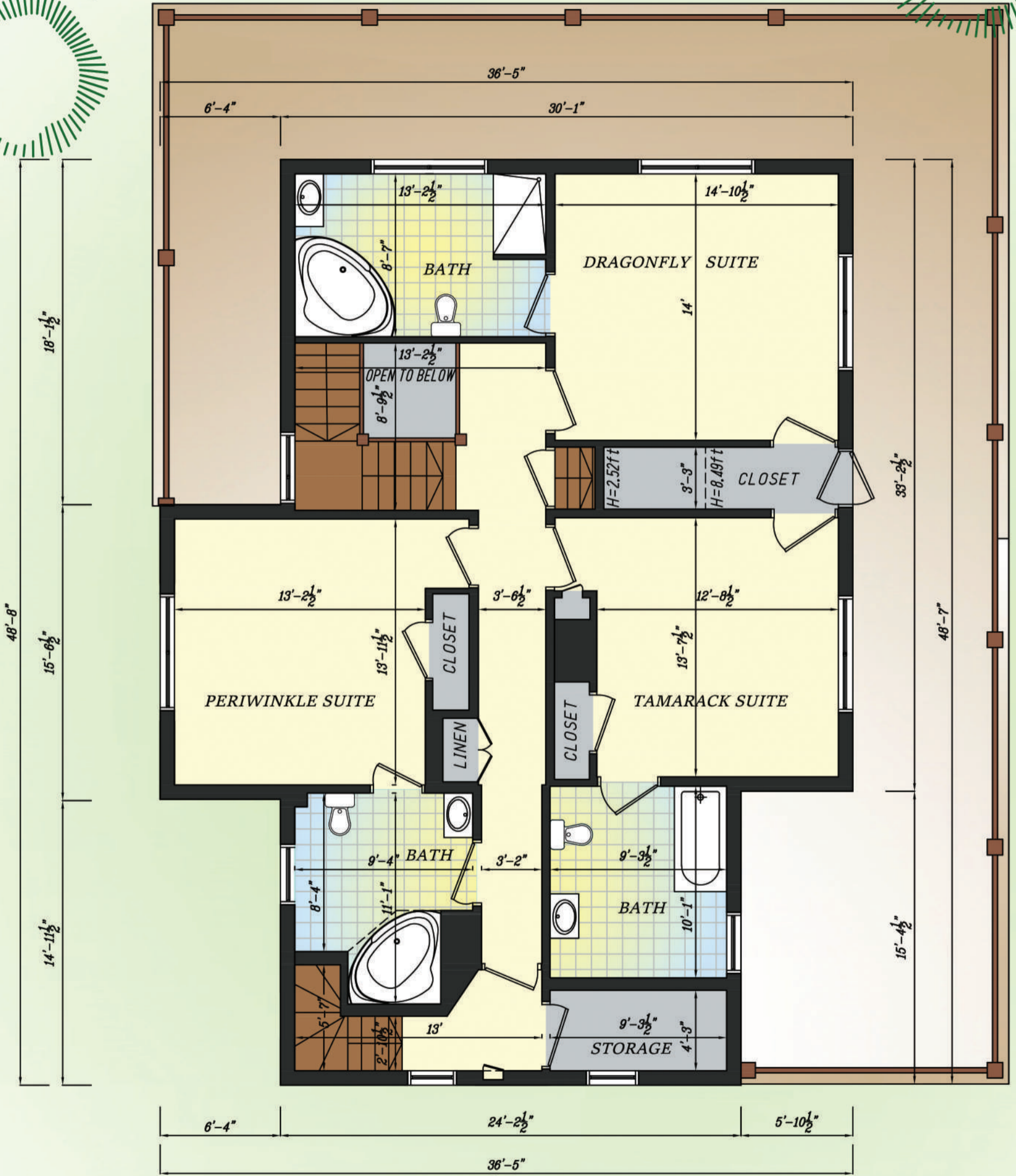
Upper Level Floor Plan Alicion Bed & Breakfast 66 McDonald Street Lunenburg, NS
